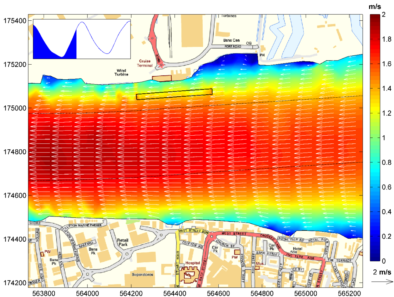
Figure 17.22: Essex Project Site Baseline Hydrodynamic showing current magnitude at time peak flood tide.
